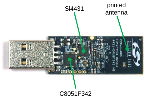
Figure 3. EZRadioPRO Dongle (plastic removed)
